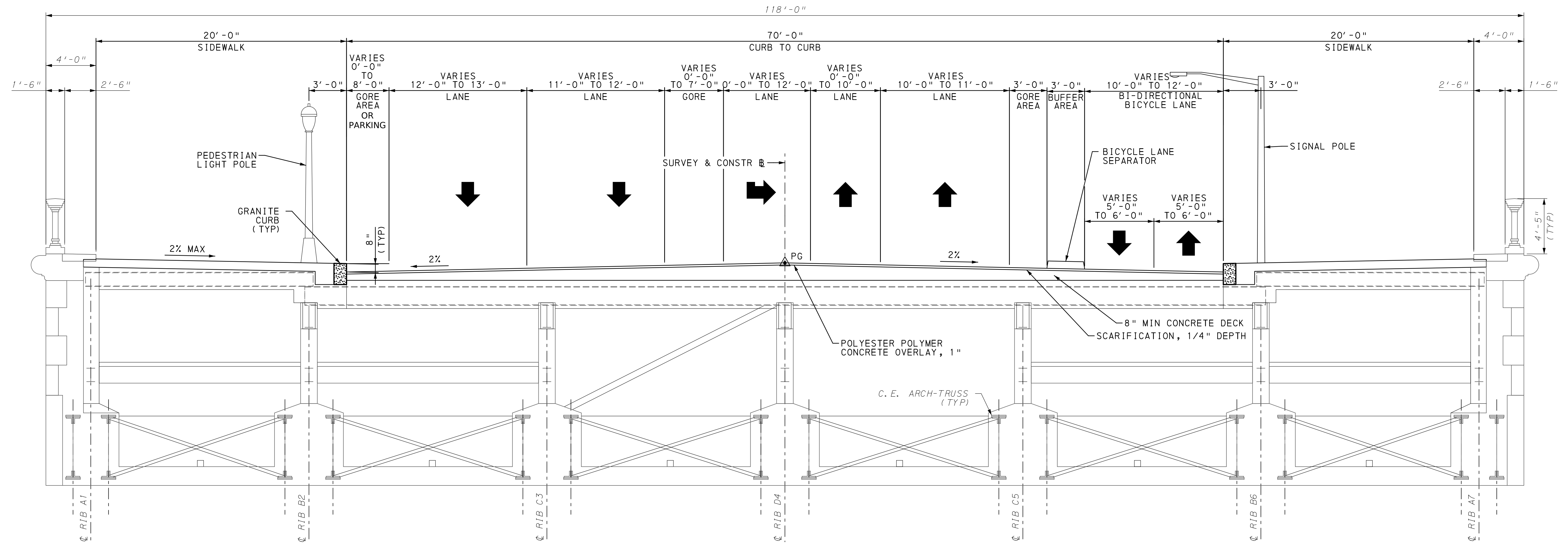
MARKET STREET OVER SCHUYLKILL RIVER TYPICAL SECTION - SR 3010 LOOKING EAST NOT TO SCALE
